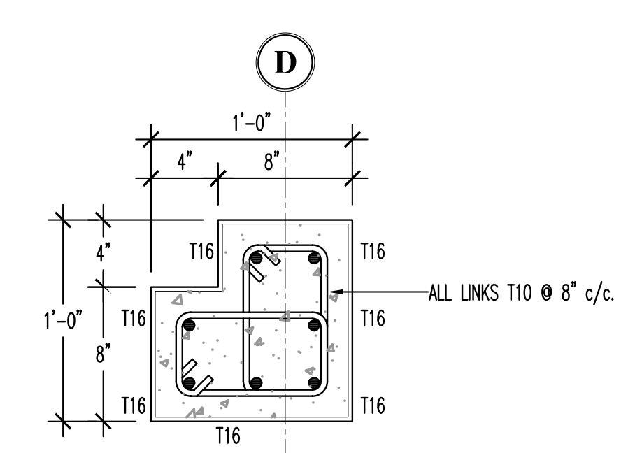
R.C. STIFFENER DETAIL (Ws1) SCALE: 1-1/2"=1'-0"
