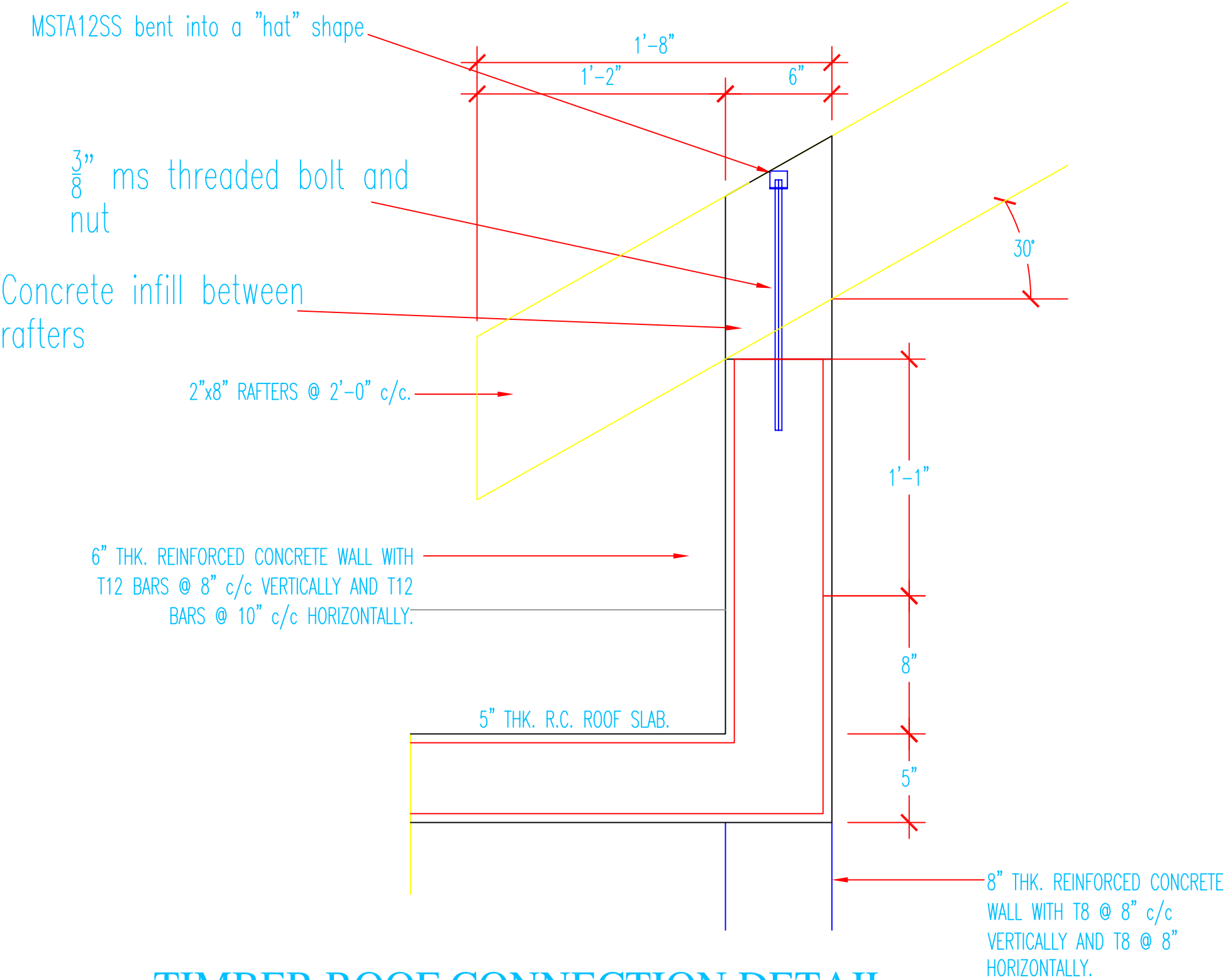
TIMBER ROOF CONNECTION DETAIL
